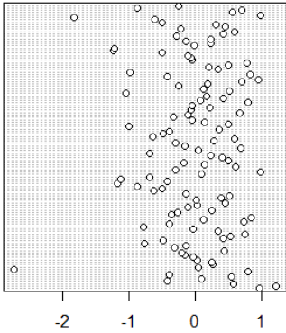
(b) Residuals
