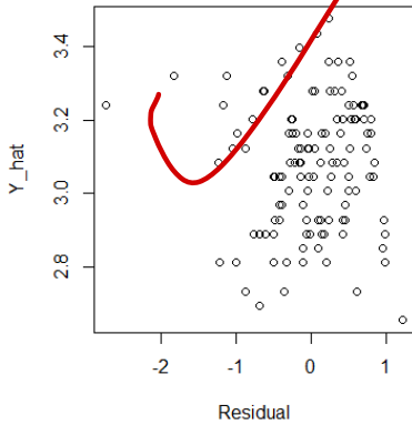
(c) Residuals
