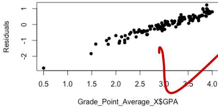
Residual Plot against X
